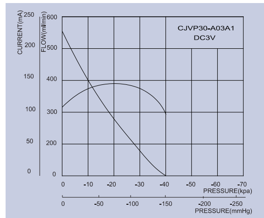
產品特性圖 Performance Curve
